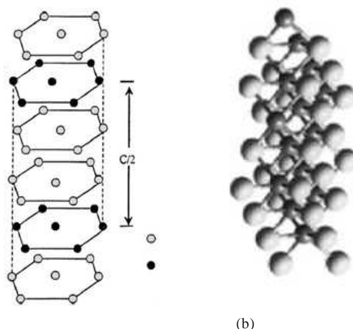
Figure (a) Layered crystal structure of NbSe 2 ( Se atoms; Nb atoms) and (b) Structure of the transition metal dichalcogenides 2H-NbS 2
